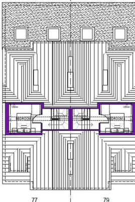
SECOND FLOOR PLANS 15m² GIA PER DWELLING
