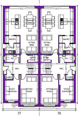
GROUND FLOOR PLANS 98m² GIA PER DWELLING
