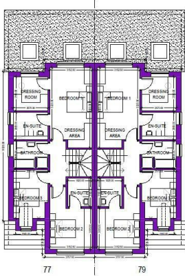
FIRST FLOOR PLANS 71m² GIA PER DWELLING
